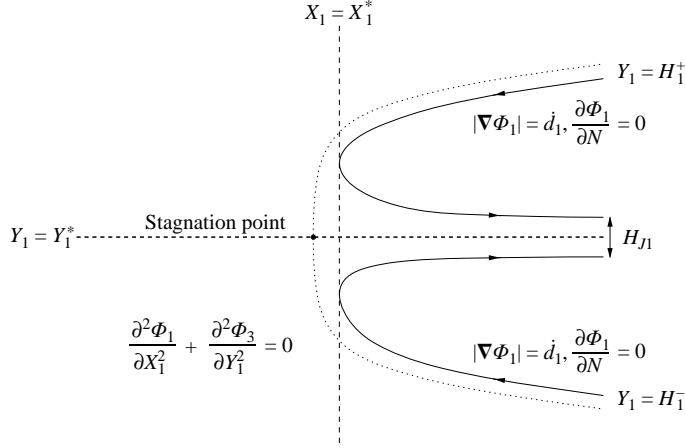
FIGURE 16. The leading-order right-hand jet root problem for t = O(\epsilon^2) ; \partial/\partial N denotes the outward normal derivative. In addition, the far-field conditions are W_1 \sim -\dot{d}_1 Z_1 + iS_1 Z_1^{1/2} as |Z_1| \rightarrow \infty and H_1^\pm \sim \pm S_1 X_1^{1/2}/\dot{d}_1 as X_1 \rightarrow \infty , where S_1 = O(1) is defined in the text.
